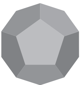
정십이면체 Dodecahedron
